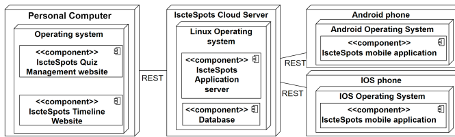
Fig. 3. IscteSpots UML deployment diagram
