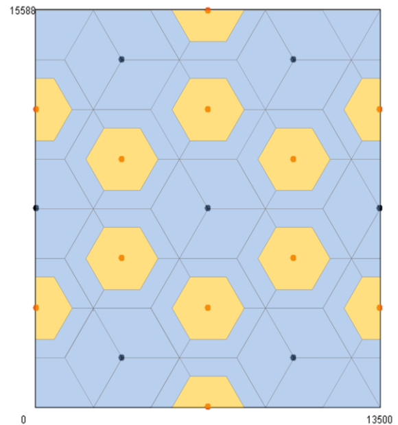
Figure 7. Coverage of Fixed Relays, and Base Stations, R=2250m.
