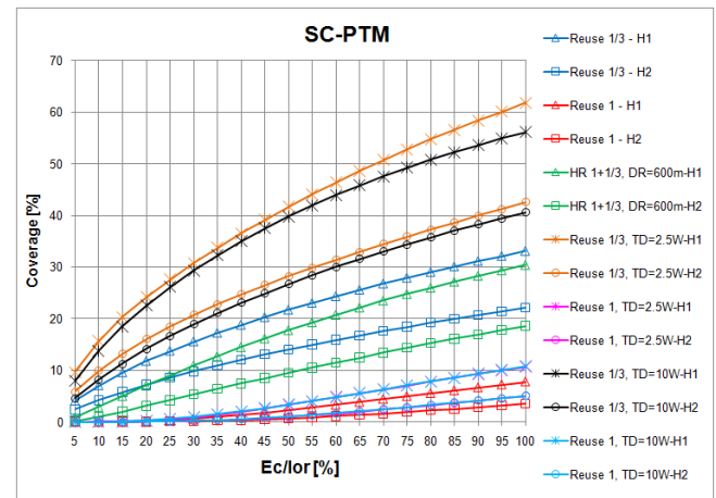
Figure 6. Coverage vs Ec/Ior SC-PTM (1RL) scenario, 16-HQAM, coding rate 3/4 , R=2250m
