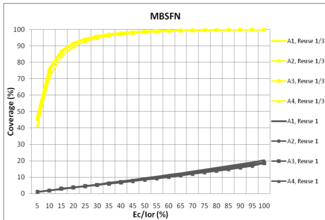
Figure 17. 4x4MIMO coverage (%) vs. E_c/I_{or} (%), for MBSFN scenario, coding rate \frac{3}{4} , R=2250m
