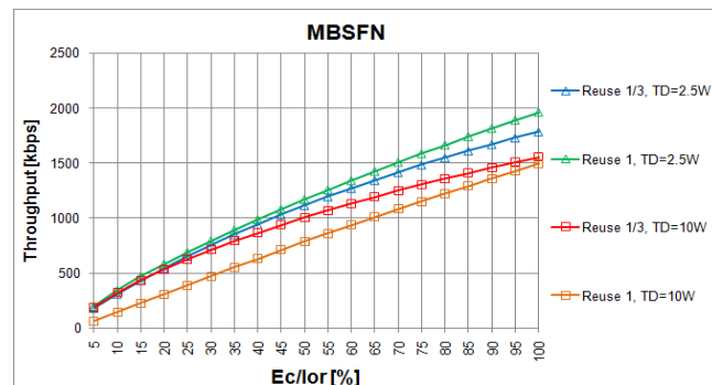
Figure 33. Throughput vs Ec/Ior for MBSFN, 16-HQAM, coding rate \frac{3}{4} , Relay Stations.
