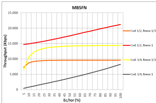
Figure 37. 4x4MIMO Throughput vs E_c/I_{or} for MBSFN scenario
