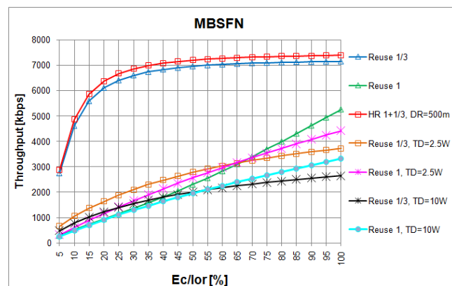
Figure 32. Throughput vs Ec/Ior for MBSFN 16-HQAM, coding rate \frac{3}{4} , Base Stations.
