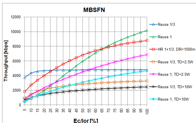
Figure 30. Throughput vs Ec/Ior for MBSFN 16-HQAM, coding rate \frac{1}{2} , Base Stations.
