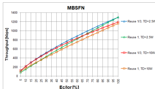
Figure 25. Throughput vs Ec/Ior for MBSFN, 64-HQAM, coding rate \frac{3}{4} , Relay Stations.
