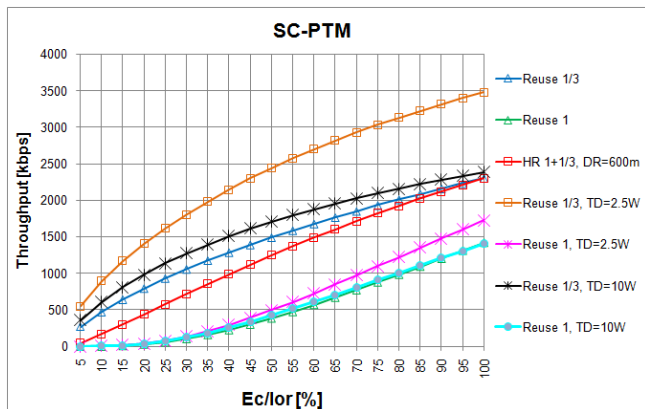
Figure 28. Throughput vs Ec/Ior for SC-PTM 16-HQAM, coding rate \frac{3}{4} , Base Stations.
