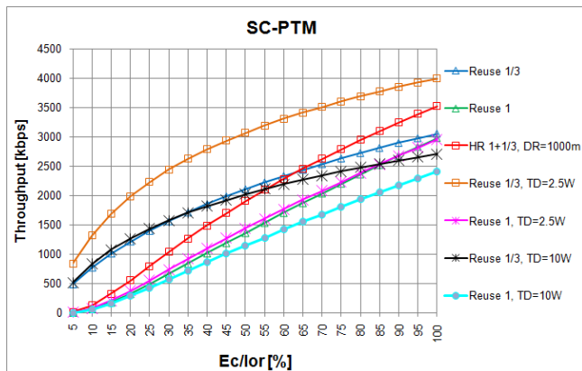
Figure 18. Throughput vs E_c/I_{or} for SC-PTM 64-HQAM, coding rate \frac{1}{2} , Base Stations.
