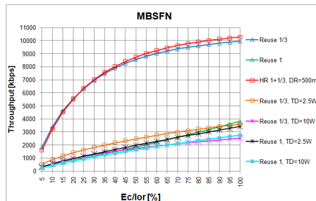
Figure 24. Throughput vs Ec/Ior for MBSFN 64-HQAM, coding rate \frac{3}{4} , Base Stations.
