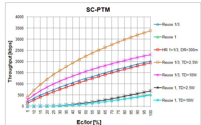
Figure 20. Throughput vs E_c/I_{or} for SC-PTM 64-HQAM, coding rate \frac{3}{4} , Base Stations.
