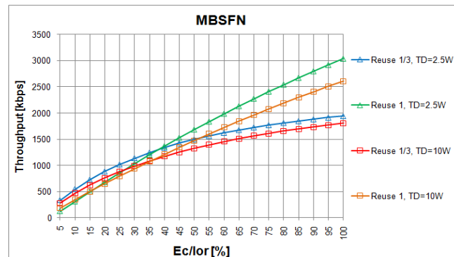
Figure 31. Throughput vs Ec/Ior for MBSFN, 16-HQAM, coding rate \frac{1}{2} , Relay Stations.
