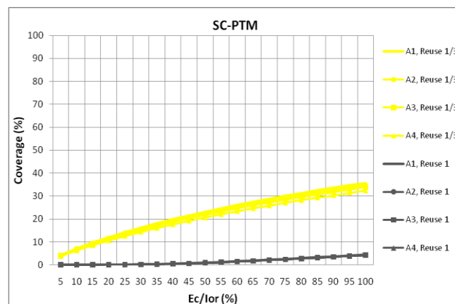
Figure 15. 4x4MIMO coverage (%) vs. E_c/I_{or} (%), for SC-PTM scenario, coding rate \frac{3}{4} , R=2250m
