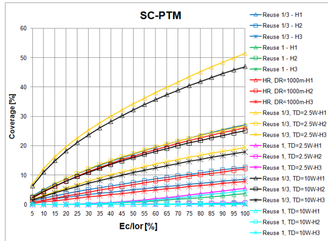
Figure 4. Coverage vs Ec/Ior SC-PTM (1RL) scenario, 64-HQAM, coding rate 3/4 , R=2250m
