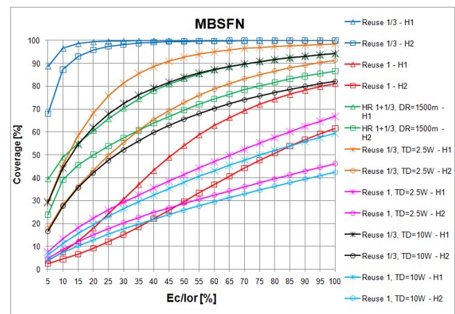
Figure 10. Coverage vs E_c/I_{or} for MBFSN scenario, 16-HQAM, coding rate \frac{1}{2} , R=2250m
