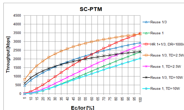
Figure 26. Throughput vs Ec/Ior for SC-PTM 16-HQAM, coding rate \frac{1}{2} , Base Stations.
