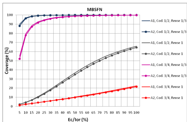
Figure 13. 2x2MIMO coverage (%) vs. E_c/I_{or} (%), for MBSFN scenario, R=2250m
