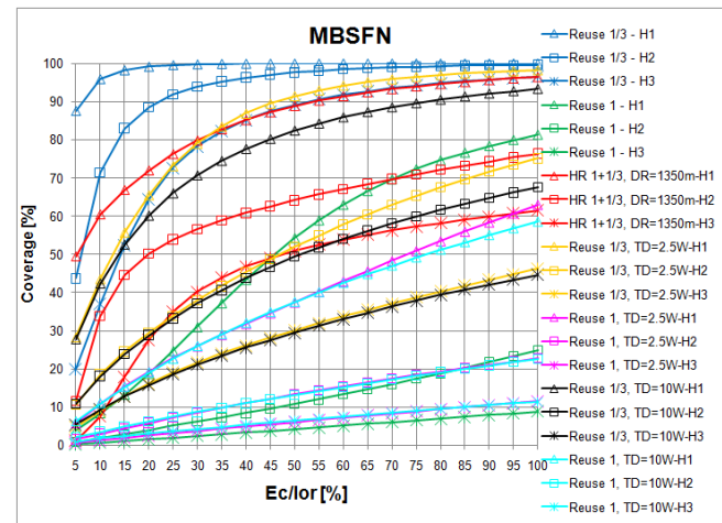
Figure 8. Coverage vs E_c/I_{or} for MBFSN scenario, 64-HQAM, coding rate \frac{1}{2} , R=2250m
