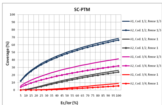
Figure 12. 2x2MIMO coverage (%) vs. E_c/I_{or} (%), for SC-PTM scenario, R=2250m
