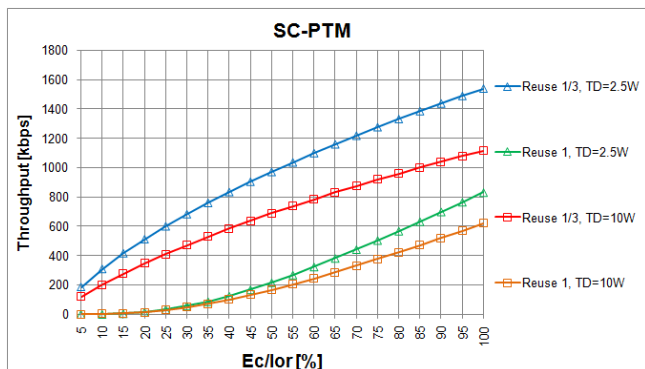
Figure 29. Throughput vs Ec/Ior for SC-PTM, 16-HQAM, coding rate \frac{3}{4} , Relay Stations.
