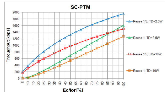
Figure 19. Throughput vs E_c/I_{or} for SC-PTM, 64-HQAM, coding rate \frac{1}{2} , Relay Stations.
