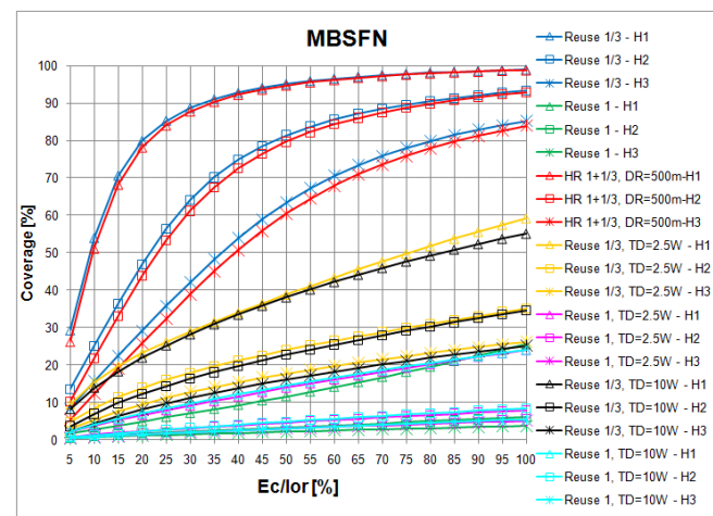
Figure 9. Coverage vs E_c/I_{or} for MBFSN scenario, 64-HQAM, coding rate \frac{3}{4} , R=2250m
