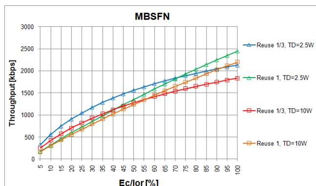
Figure 23. Throughput vs Ec/Ior for MBSFN, 64-HQAM, coding rate \frac{1}{2} , Relay Stations.
