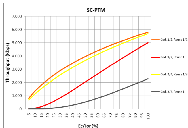
Figure 36. 4x4MIMO Throughput vs Ec/Ior for SC-PTM scenario
