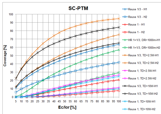
Figure 5. Coverage vs Ec/Ior SC-PTM (1RL) scenario, 16-HQAM, coding rate 1/2 , R=2250m
