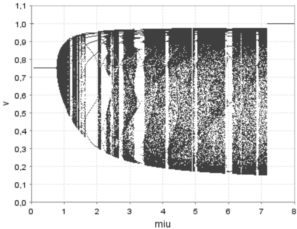
Figure 3: Bifurcation diagram (v_t; \mu) .
