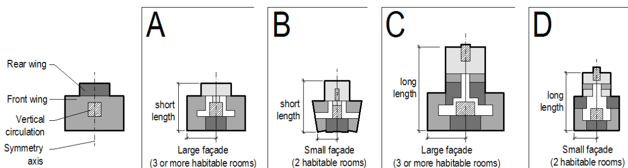
Figure 7 – Types of “rabo-de-bacalhau” dwellings
