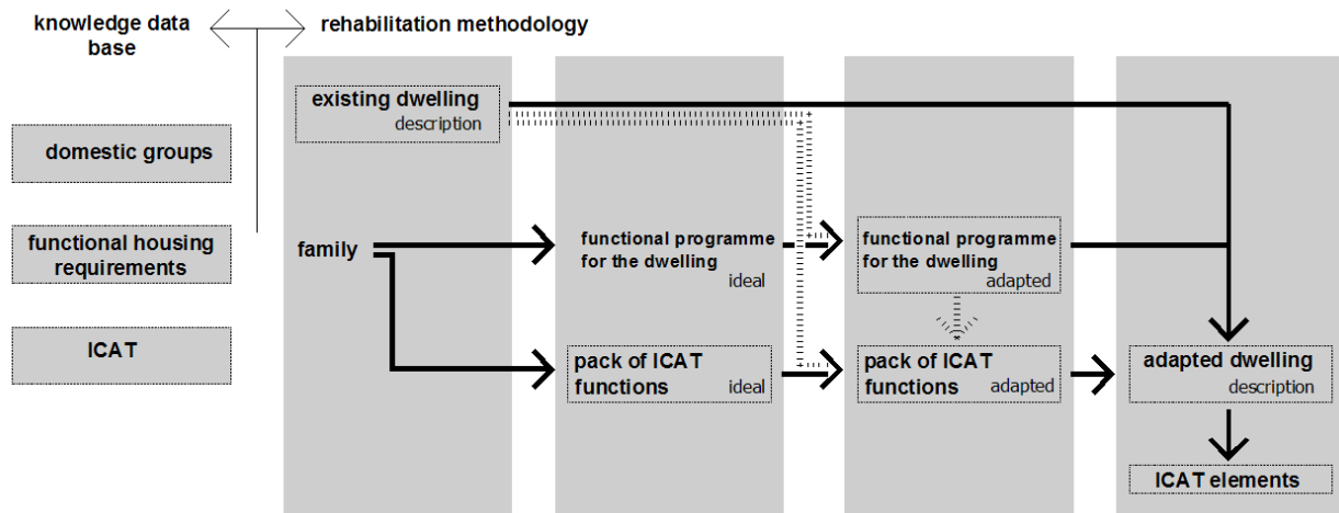
Figure 1 – Basic steps in the planned rehabilitation methodology.
