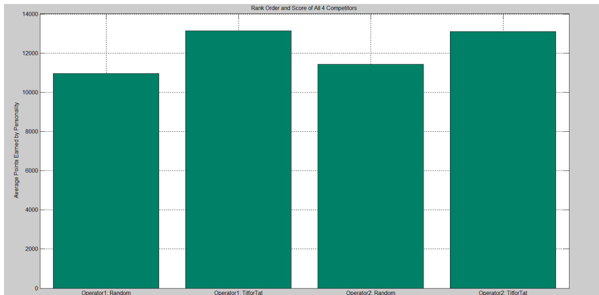
Figure 6: Outcomes of a finite repeated prisoner's dilemma game using two distinct strategies.
