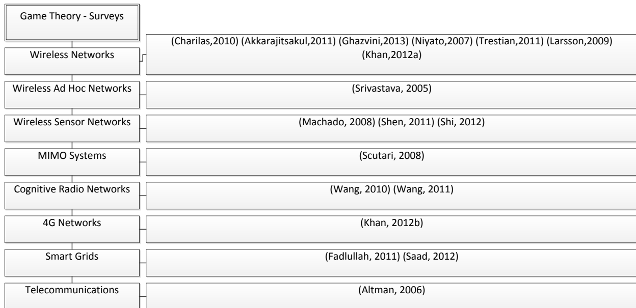
Figure 7: Summary of Game Theory Surveys.
