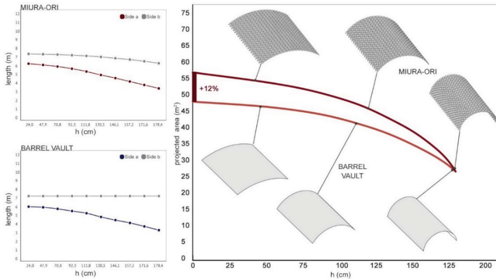
Figure 6. Geometric comparison between a curved Miura-ori tassellation and a barrel vault: (a) side ratio a/b ; (b) projected area variation throughout the folding phase.
