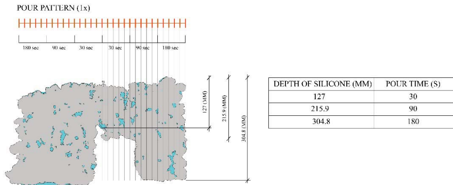
Figure 6. Arch test data.
