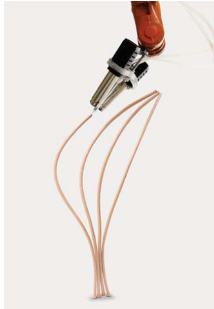
Figure 1. Plastic mix robotic extrusion creating gravity defying structures. Source: https://www.dezeen.com/2013/05/17/mataerial-3d-printer-by-petr-novikov-sasa-jokic-and-joris-laarman-studio/
