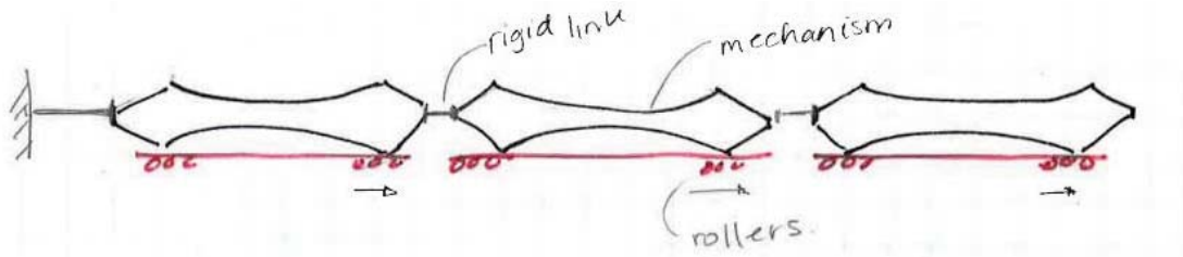
Figure 16. Schematic representation of a linkage system to prevent accumulation of resistance during actuation of the module.
