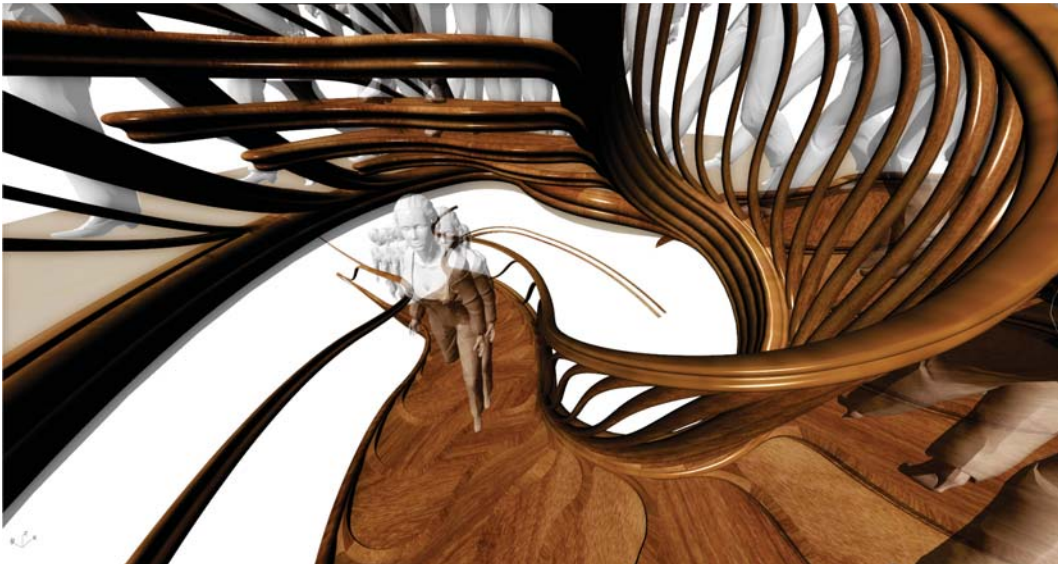
Figure 3. StairStalk
