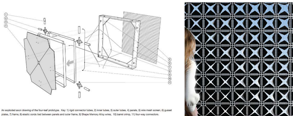
Figure 1. An exploded diagram of the four-leaf prototype assembly. Photograph of the possible module layout. Diagram and photo courtesy of Andrew Payne.
