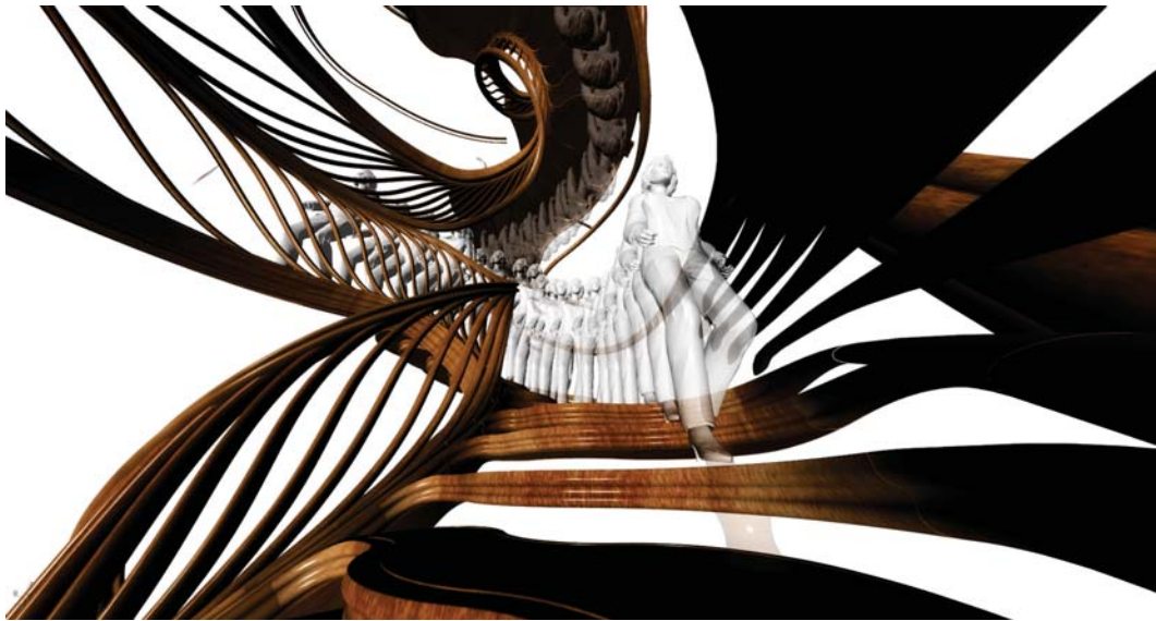
Figure 1. StairStalk
